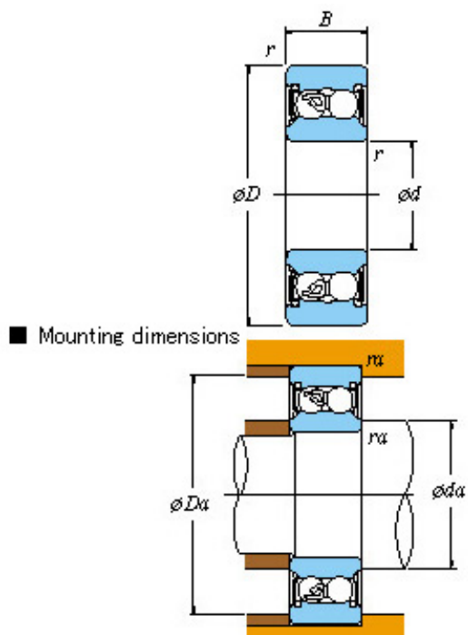
23092RS Bearing 2D drawings and 3D CAD models
